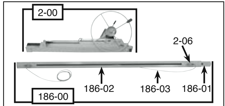
Extension Unit 186-00
